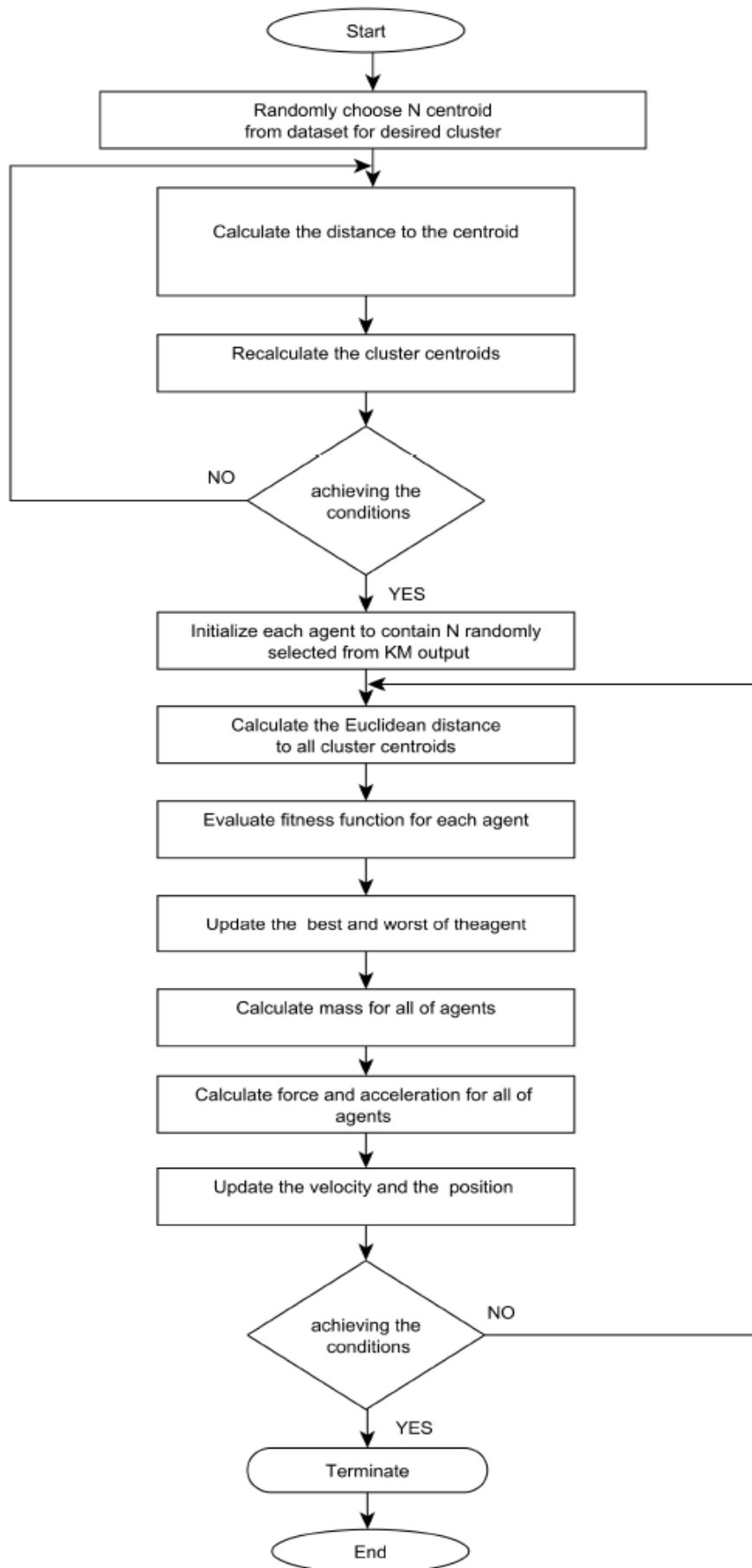
Fig. 1.KM-GSA Hybrid Algorithm
